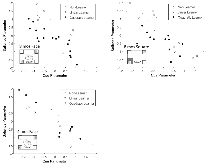
Figure 6: Weights for cued and saliency locations across conditions labeled by learning score. The negative slope is a direct consequence of our null function, but the relationship of the parameters to learning rates is not. In fact, weighting the cue over the salient locations led to better learning in both 8 months conditions, with an eventual decline in the face condition. Two distinct clusters of learners were found among the 4-month-olds.
