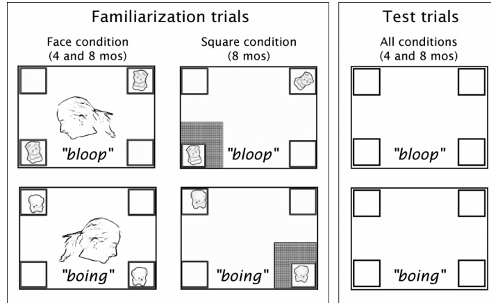
Figure 1: Familiarization and test trials from the Face and Square cueing conditions from [1]. The stimuli were in full color; the frames were white and presented on a black background. The hatched lines represent a red flashing square.
